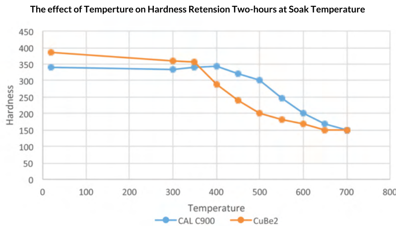
Chart 1 - Hardness Curve verses Temperature
